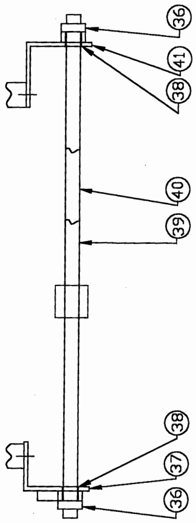
DWG. NO. NLE-A76VLRC (NEW STYLE) MODEL E7RC/EPRC L.H. CONTROL LABELER PRESSURE PASTE SYSTEM DRIVE AND SUPPORT ASSFMRI Y
