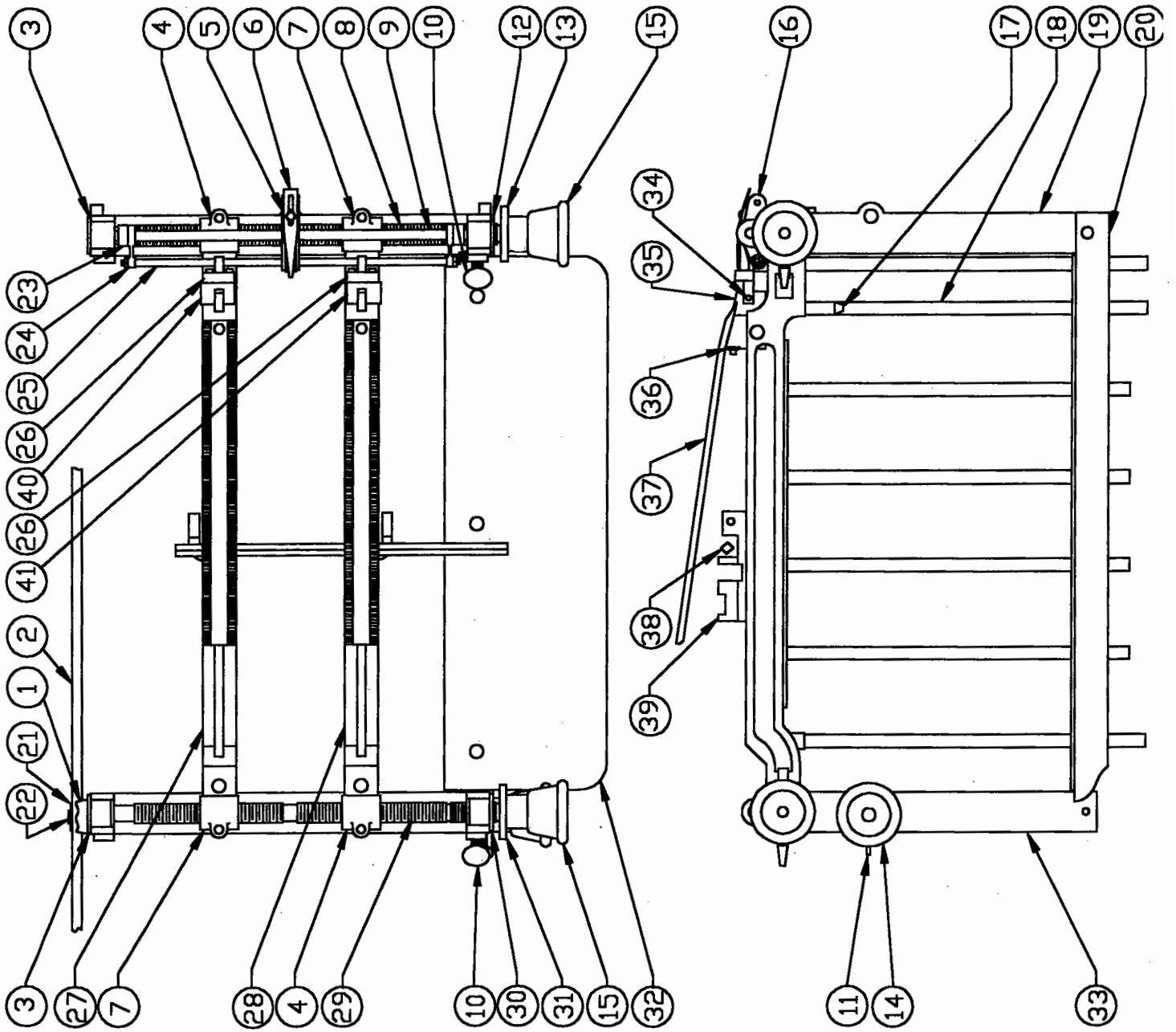
DWG. NO. NLE-A2100SRC MODEL E5RC L.H. CONTROL LABELER ABEL BED RISER & GUIDE ASSEMBLY
