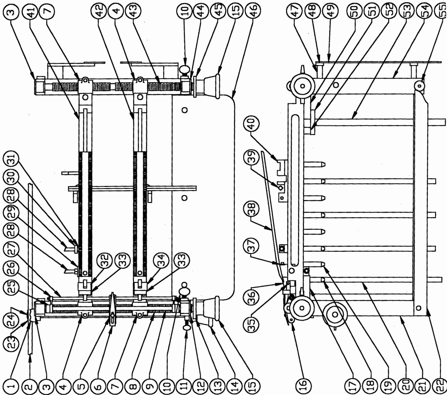
DWG. NO. NLE-A2100SCT MODEL E5 LABELER CONTINUOUS FEED (TOGGLE FINGER TYPE) LABEL BED RISER & GUIDE ASSEMBLY
