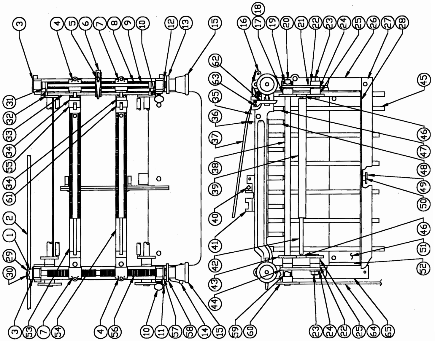
DWG. NO. NLE-A2100SCFRC MODEL ESRC L.H. CONTROL LABELER CONTINUOUS FEED (FLIGHT BAR TYPE) LABEL BED RISER & GUIDE ASSEMBLY
