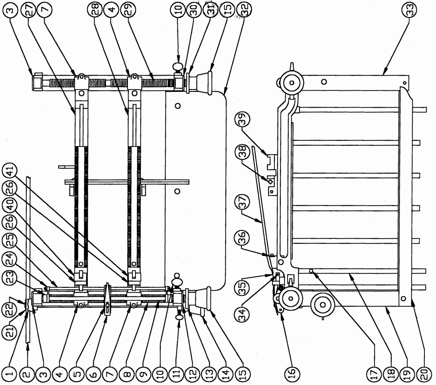
DWG. NO. NLE-A2100S MODEL E5 LABELER LABEL BED RISER & GUIDE ASSEMBLY
