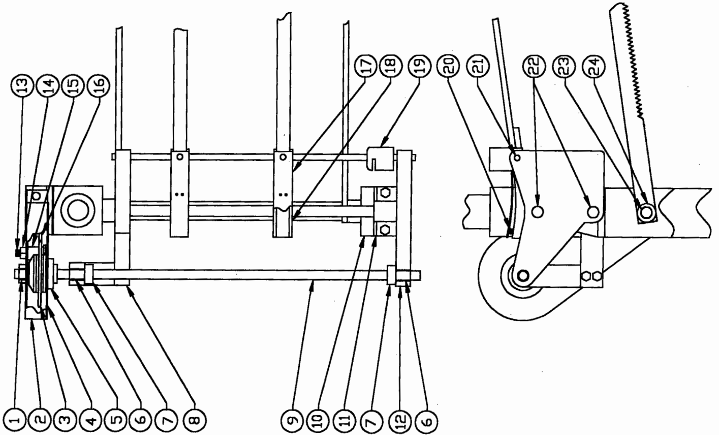
DWG. NO. NLE-A130 MODEL E5/E7/EP LABELER BOOSTER INFEEED DRIVF ASSFMRI Y
