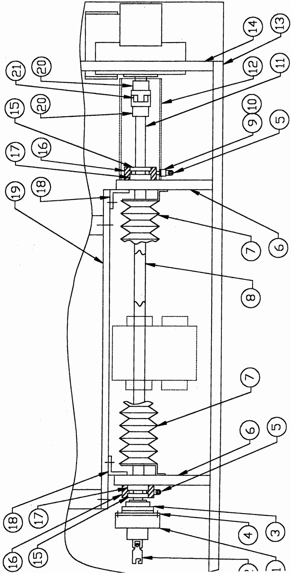
DWG. NO. NAL-A74PSRC MODEL A5RC L.H. CONTROL LABELER WIRE BELT PASTE DRIVE AND SUPPORT ASSEMBLY
