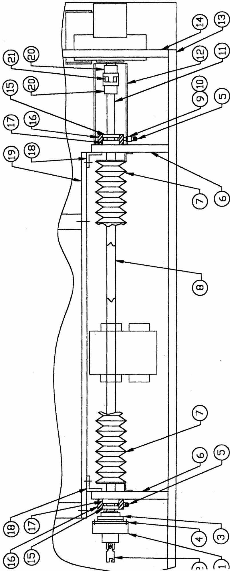
DWG. NO. NAL-A72PLRC MODEL A7RC/APRC L.H. CONTROL LABELER WIRE BELT PASTE DRIVE AND SUPPORT ASSEMBLY
