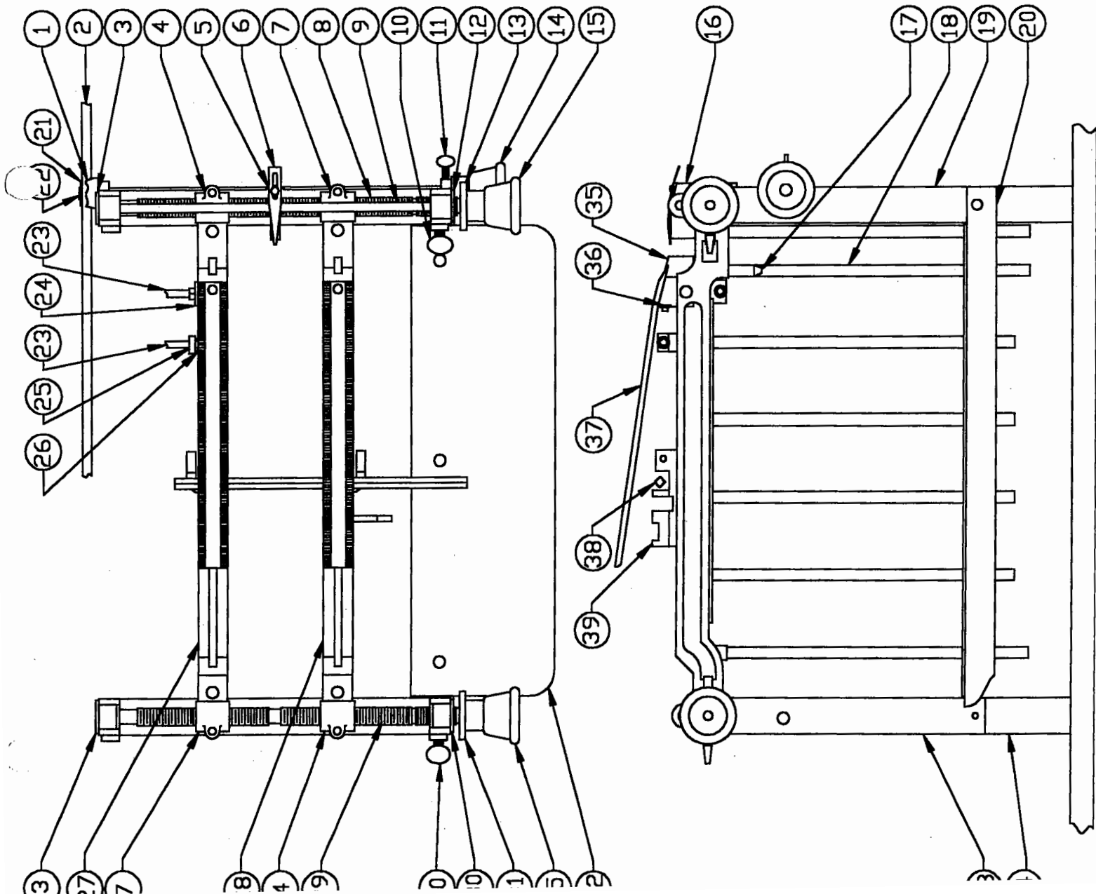
DWG. NO. NAL-A2100SRC MODEL A5RC L.H. CONTROL LABELER LABEL BED RISER & GUIDE ASSEMBLY
