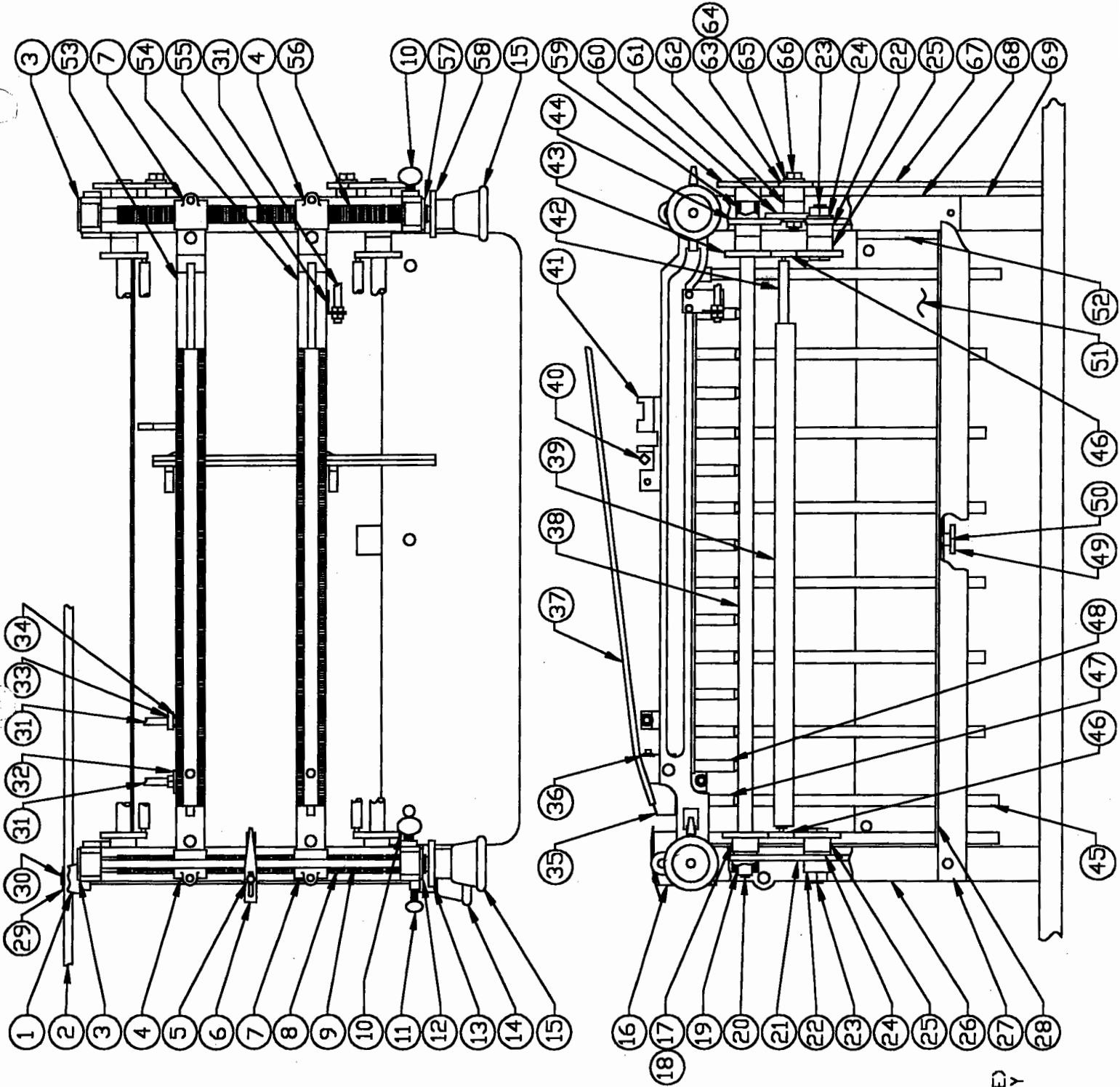
DWG. NO. NAL-A2100LCF MODEL A7/AP LABELER CONTINUOUS FEED (FLIGHT BAR TYPE) LABEL BED RISER & GUIDE ASSEMBLY
