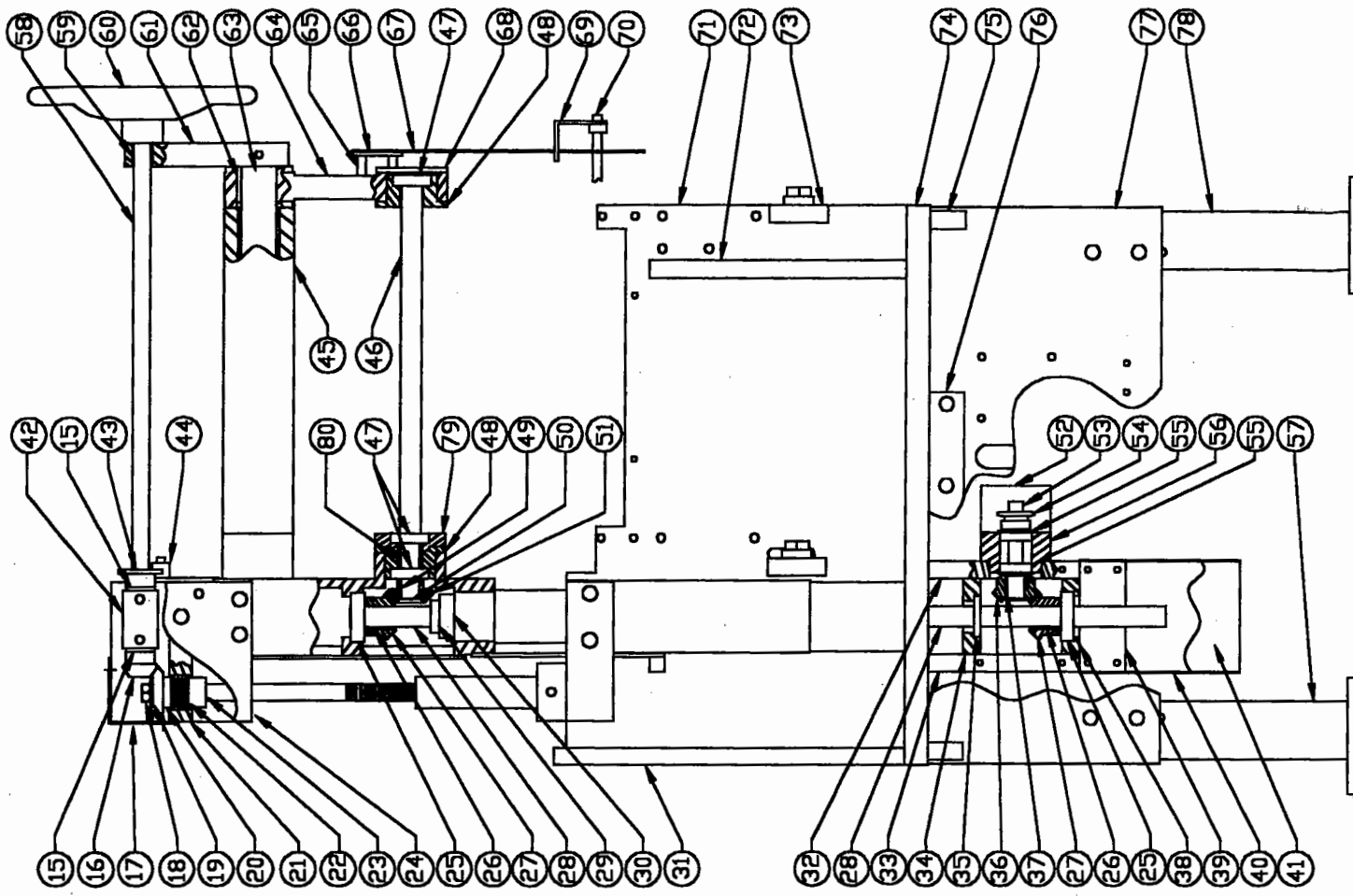
DWG. NO. NAL-A19S/BOOSTER MODEL A5 LABELER FEED END COLUMN SUPPORT WITH BOOSTER DRIVE ASSY.
