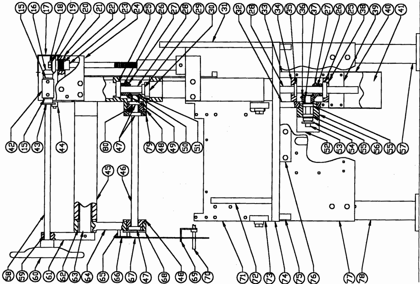
DWG. NO. NAL-A19LRC/BOOSTER MODEL A7RC/APRC L.H. CONTROL LABELER FEED END COLUMN SUPPORT WITH BOOSTER DRIVE ASSY.
