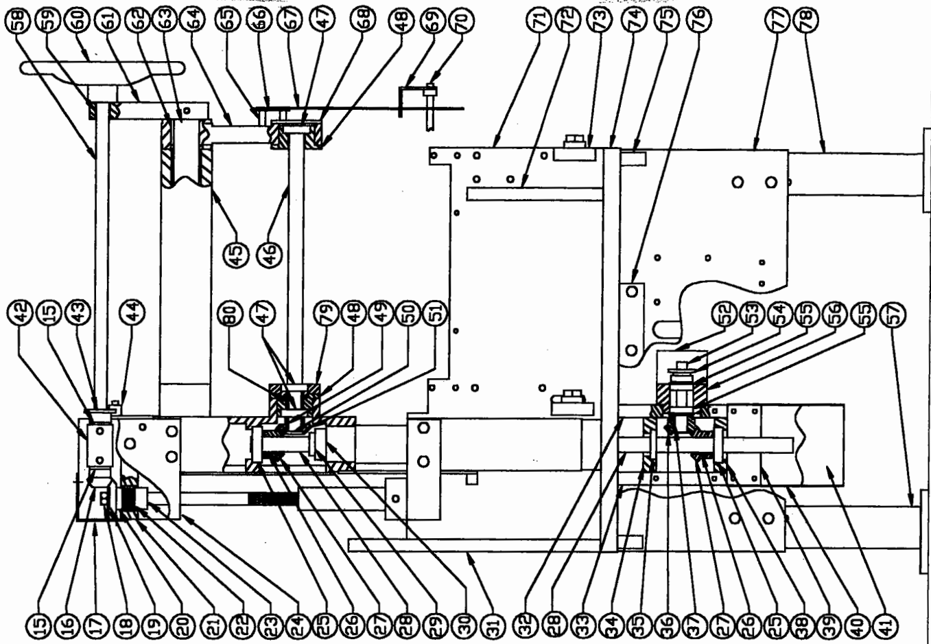
DWG. NO. NAL-A19L/BOOSTER MODEL A7/AP LABELER FEED END COLUMN SUPPORT WITH BOOSTER DRIVE ASSY.
