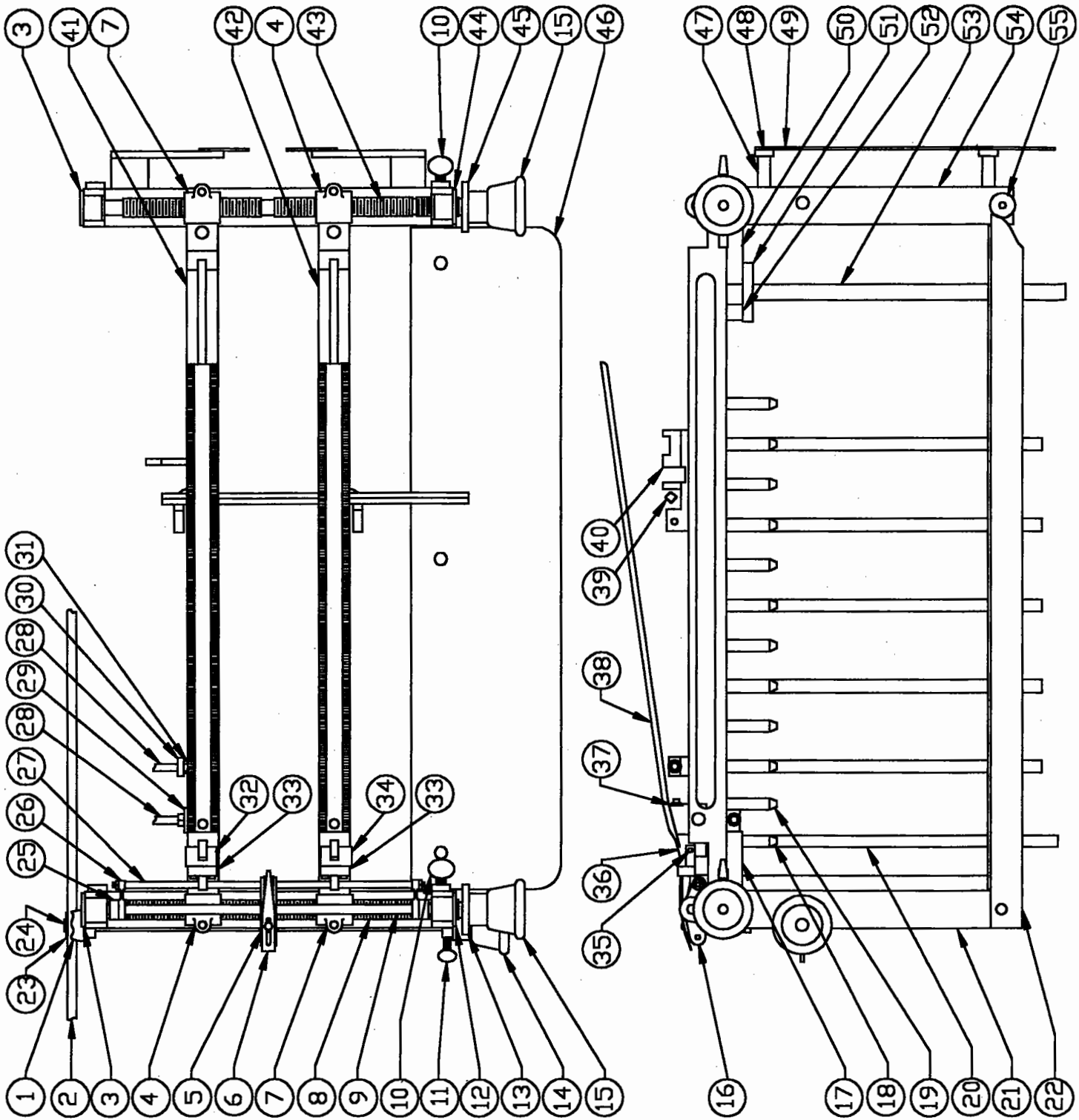
DWG. NO. NA-A2100LCT MODEL SA7 LABELER CONTINUOUS FEED (TOGGLE FINGER TYPE) LABEL BED RISER & GUIDE ASSEMBLY
